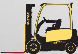
J2.2XN, J2.5XN, J3.0XN, J3.5XN 2 200-3 500 KG @ 500 MM
