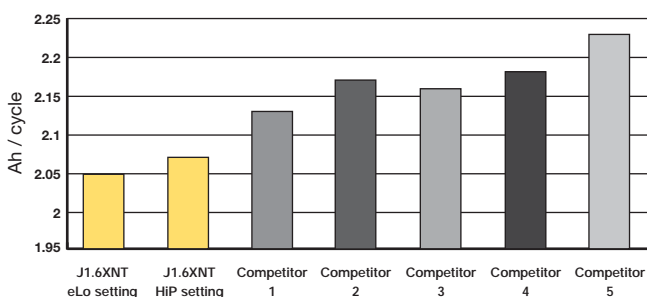
VDI 2198 (2002) Test Cycle (JXNT)
