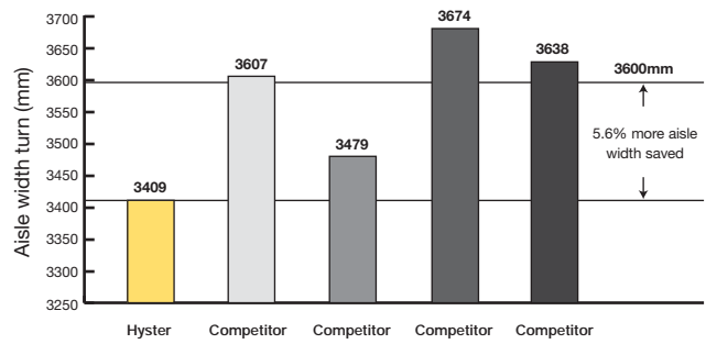
Euro Pallet 800 x 1200mm
